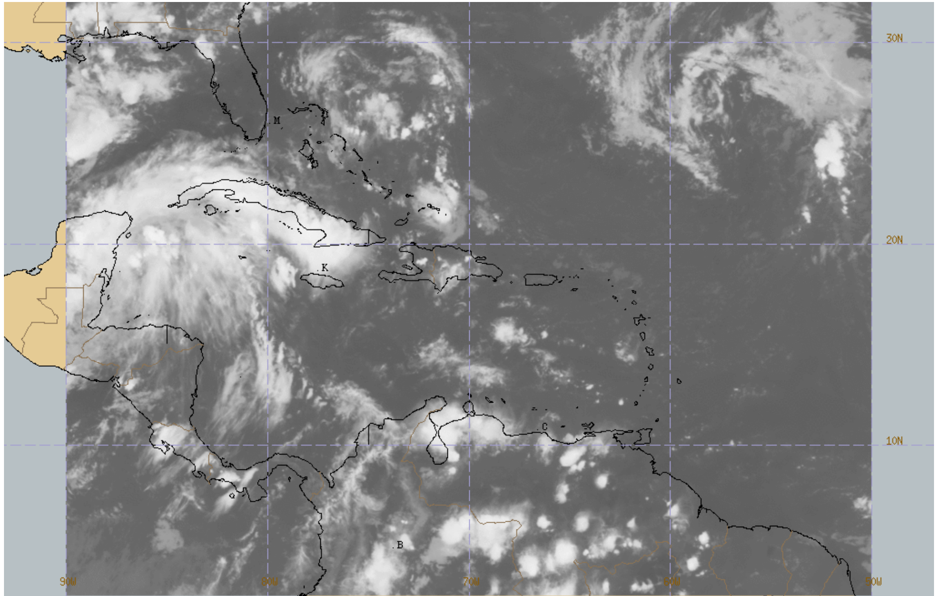
Satellite DirectMet Caribatl INFRARED1 Obs Mon 21 Aug 2017 2315z
